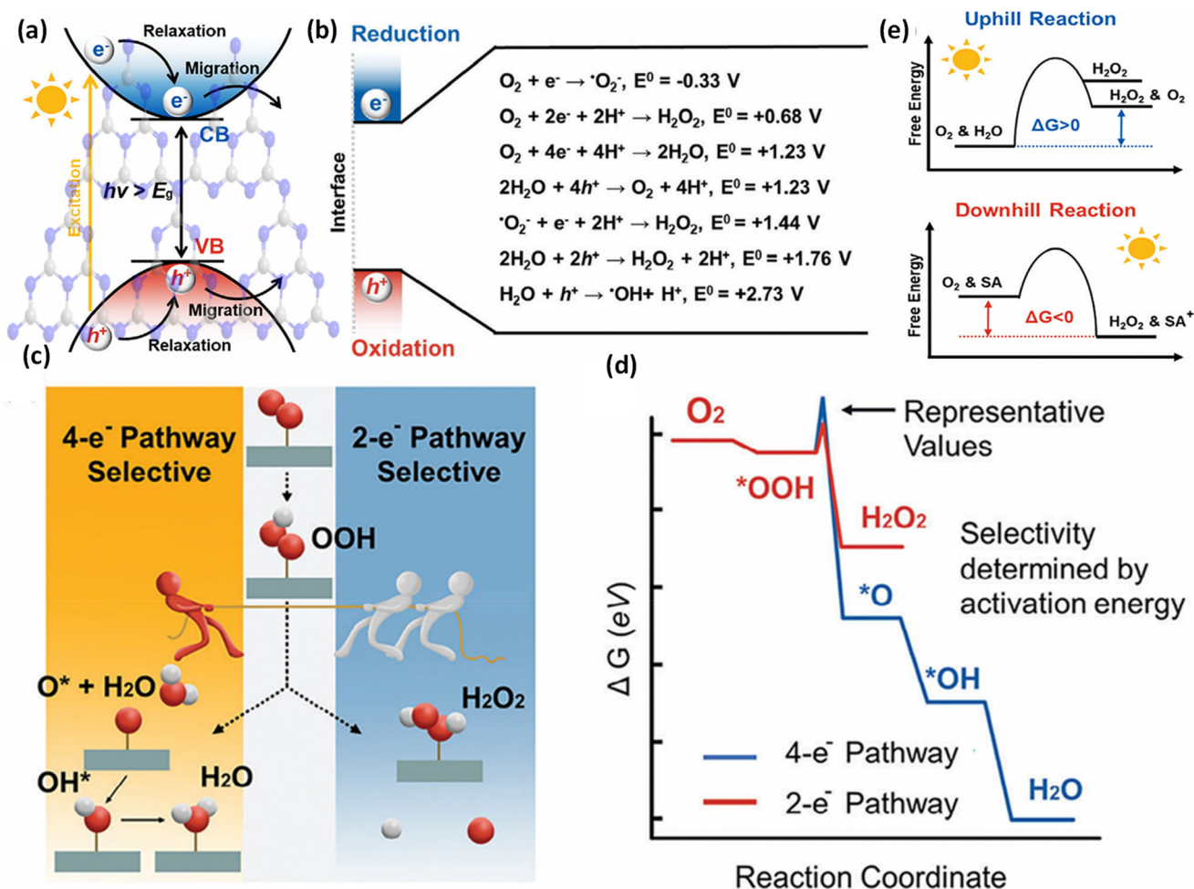
Fig. 22 Illustrations of various stages of (a) photoexcitation and transfer of charge carriers. (b) Surface redox reaction processes relevant to solar \text{H}_2\text{O}_2 formation. (c and d) The competition between two-electron and four-electron routes in the oxygen reduction reaction, represented by a free energy diagram. (e) The concept of uphill and downhill processes in this production process. The figures are reproduced with permission from ref. 189. Copyright 2024, Wiley-VCH.
