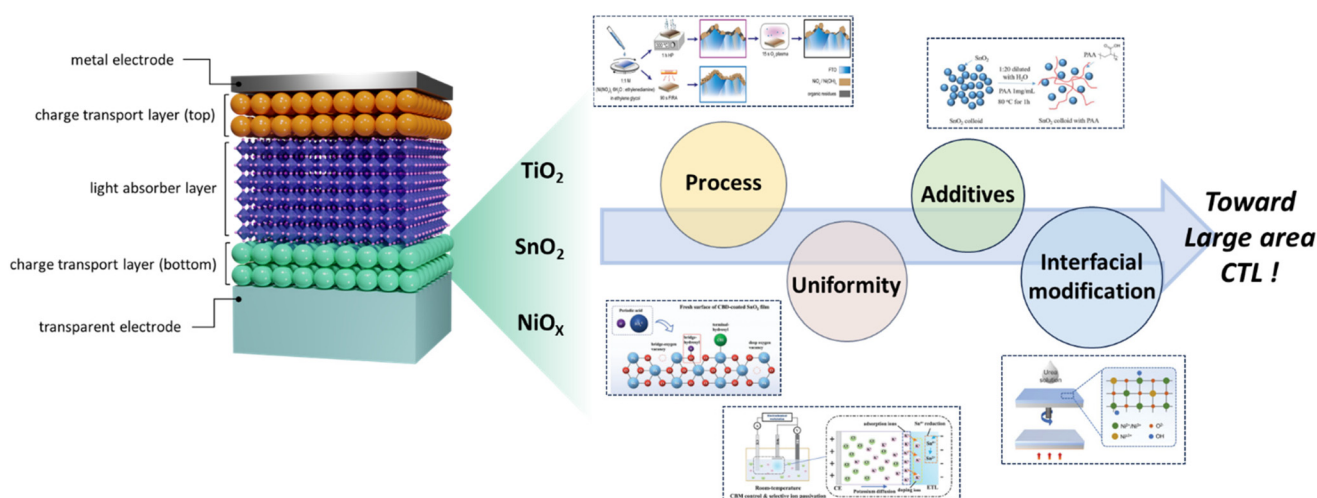
Fig. 1 Schematic PSC structure and illustration of requirements toward large-area CTL.
