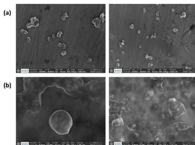
Fig. 3 (a) SEM image of MnO 2 NPs (scale bar is 500 nm; right: scale bar is 1 \mu m), (b) SEM image of PNIPAM@MnO 2 NPs (scale bar is 500 nm; right: scale bar is 1 \mu m).
