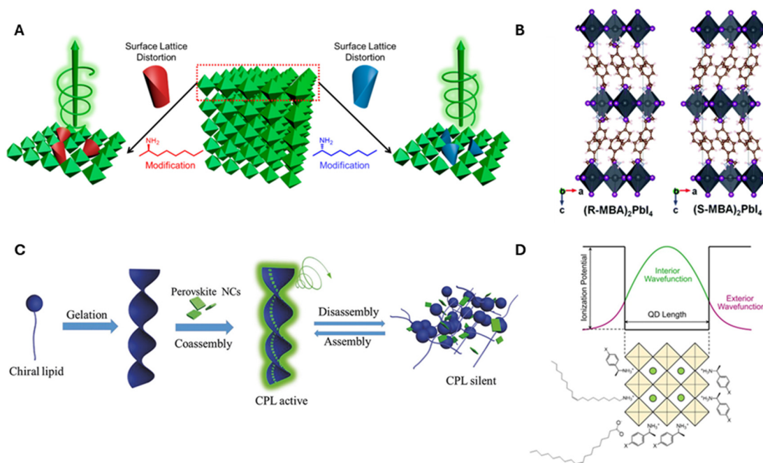
Fig. 1 Panel A shows a schematic diagram of chirality induction through surface distortion in R - and S -α-octylamine capped \text{CsPbBr}_3 NPs. Panel B shows an example of a chiral crystalline structure that can manifest upon incorporation of R and S -MBA organic cations into lead iodide perovskite octahedral sheets. Panel C shows an illustration for the induction of chirality in perovskites through the co-assembly of achiral \text{CsPbX}_3 NCs onto helical lipid structures. Panel D shows a schematic diagram for electronic chiral imprinting between chiral surface ligands and 2 nm sized \text{CsPbBr}_3 NPs through wavefunction hybridization. Panel A is adapted from ref. 27 with permission; Copyright 2019, American Chemical Society. Panel B is adapted from ref. 1 with permission; Copyright 2017, Royal Society of Chemistry. Panel C is reproduced from ref. 30 with permission; Copyright 2018, John Wiley and Sons. Panel D is reproduced from ref. 22; Copyright 2024, Springer Nature/the authors.
