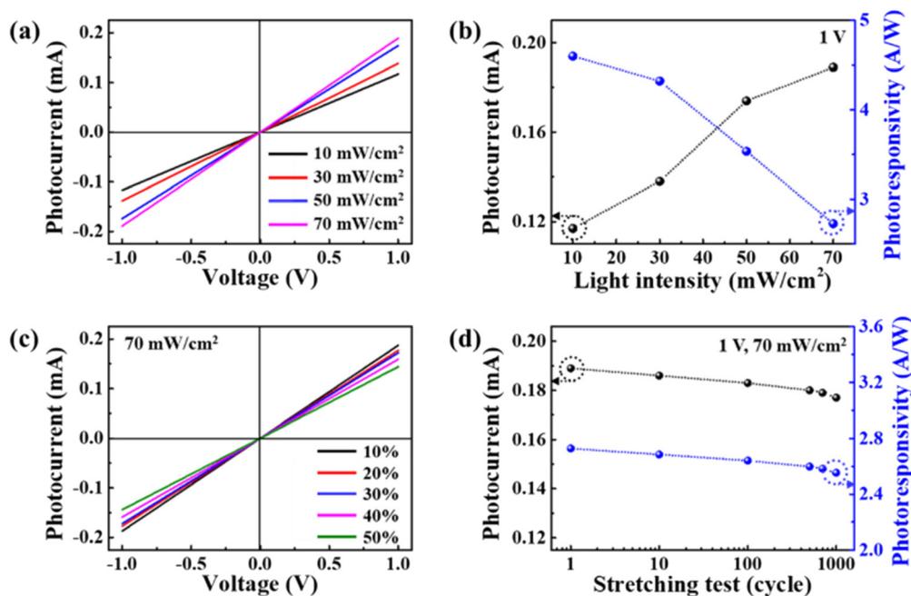
Fig. 3 (a) Characteristic I - V curves for the stretchable InN-NW photosensor at various light intensities. (b) Summary of the dependence of the photocurrent and photoresponsivity on the light intensity. (c) Characteristic I - V curves for the photosensor for the indicated strain values. (d) Summary of the photocurrent of the photosensor for the indicated number of stretching cycles.
