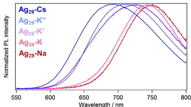
Fig. 5 PL spectra of \text{Ag}_{29}\text{-Cs} , \text{K} , \text{K}' , \text{K}'' and \text{Na} crystals.
