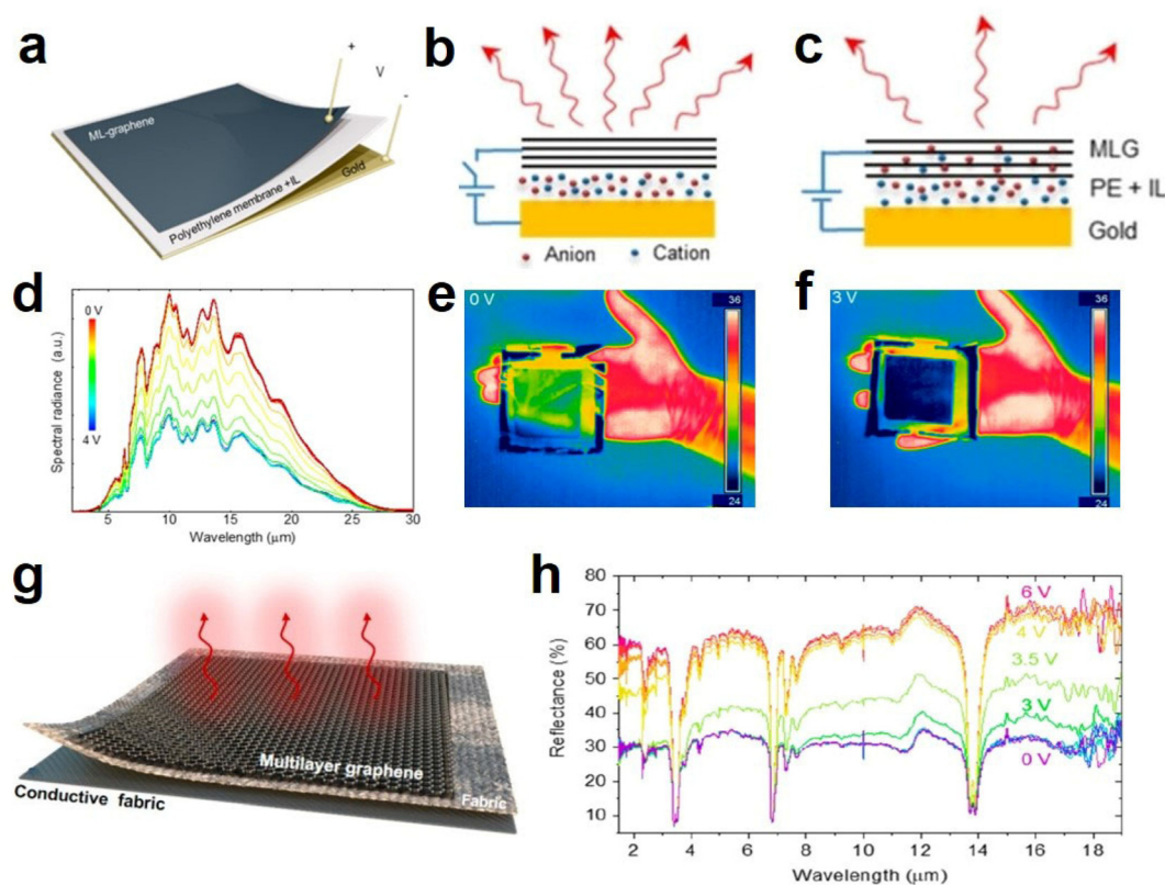
Fig. 13 (a) Structure diagram, (b and c) principal diagram of graphene-based device. (d) Spectra of the thermal radiation from the graphene-based device at voltages. (e and f) Thermal camera images of device at 0 V and 3 V. (a–f) Adapted with permission from ref. 18. Copyright 2018, American Chemical Society. (g) Schematic diagram of the textile device with various laminated layers. (h) Infrared reflectance spectra of the textile at different voltages. (g and h) Adapted with permission from ref. 19. Copyright 2020, American Chemical Society.
