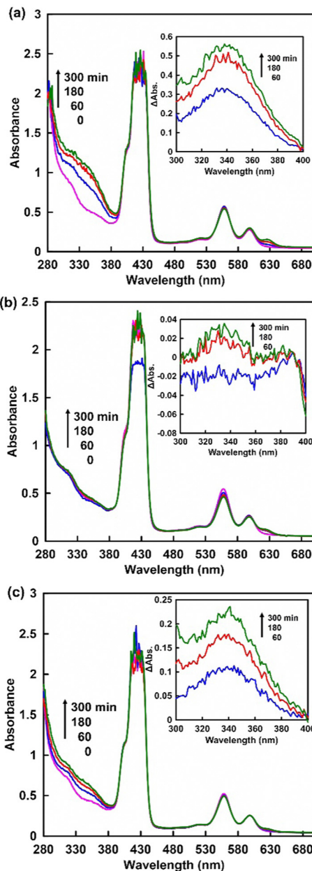
Fig. 3 UV-vis absorption spectra changes in the sample solution consisting of TEOA, ZnTPPS, Rh-PVP and NAD + analogues with irradiation. (a) NAD + , (b) NAM, (c) NMN + . Inset: Different UV-Vis absorption spectra of the sample solution from 0 min irradiation.
