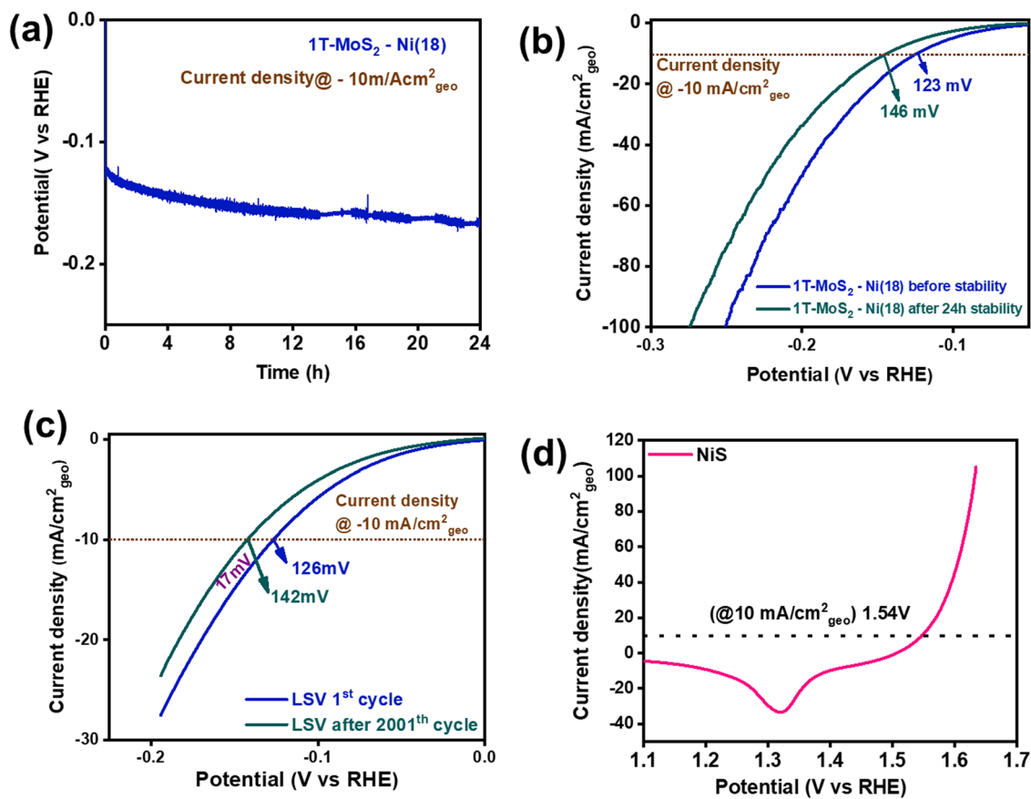
Fig. 6 (a) A 24-h-long durability study (steady state CP test) at a current density of -10\text{ mA cm}^{-2}_{\text{geo}} . (b) comparison of the cathodic polarization curves before and after the 24-h stability test. (c) ADS experiment (cyclic stability test) of 1\text{T-MoS}_2\text{-Ni}(18) towards the alkaline HER. (d) Backward anodic polarization curve (100% iR corrected) for NiS towards the alkaline OER.
