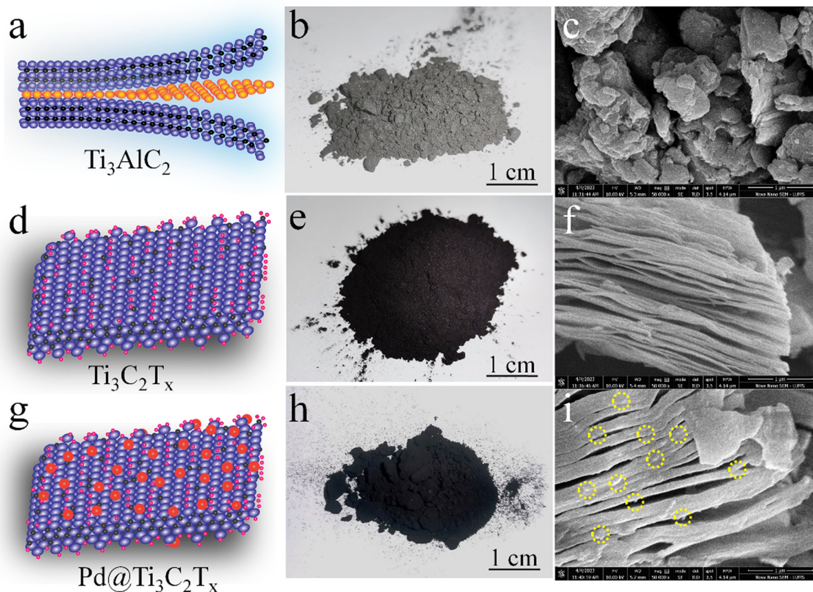
Fig. 3 (a) Schematic illustration, (b) digital photograph, and (c) SEM image of MAX (Ti 3 AlC 2 ). (d) Schematic illustration, (e) digital photograph, (f) SEM image of MXene (Ti 3 C 2 T x ). (g) Schematic illustration, (h) digital photograph, and (i) SEM image of Pd@MXene (Pd@Ti 3 C 2 T x ).
