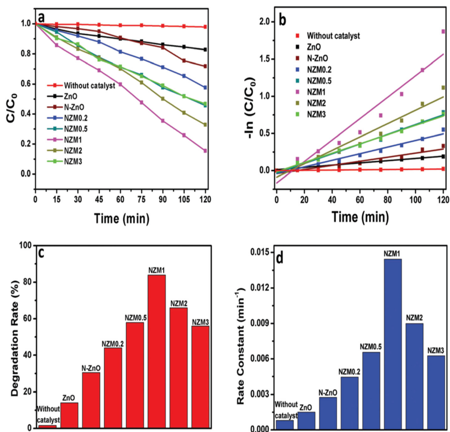
Fig. 19 (a) Kinetic curves for the degradation of TC, (b) -\ln(C/C_0) vs. time curve for the degradation of TC, (c) a histogram showing a comparative degradation rate (%) of TC under visible light illumination and (d) a bar graph showing the values of rate constants for all the photocatalysts (N-doped ZnO nanorods loaded 0.2, 0.5, 1, 2 and 3 wt% of with MoS 2 nanoflowers (MNF) are referred to as NZM0.2, NZM0.5, NZM1, NZM2, and NZM3, respectively). Reproduced from ref. 643 with permission from RSC (2017).
