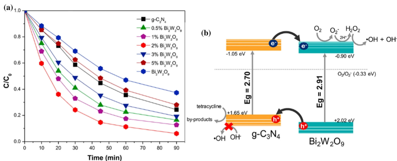
Fig. 20 (a) Photocatalytic degradation of tetracycline antibiotic ( C_0 = 10 \text{ mg L}^{-1} , \text{pH} = 4.89 ) as a function of irradiation time over Bi 2 W 2 O 9 , g-C 3 N 4 and Bi 2 W 2 O 9 /g-C 3 N 4 samples. (b) Proposed photocatalytic mechanism for the Bi 2 W 2 O 9 /g-C 3 N 4 system under solar-like irradiation. Reproduced from ref. 72 with permission of Elsevier (2020).
