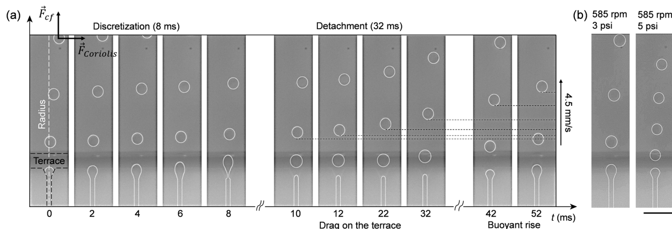
Fig. 3 Droplet generation on the centrifugal platform observed in real-time. (a) Timeline of the droplet generation process. \vec{F}_{cf} and \vec{F}_{Coriolis} are the centrifugal and Coriolis forces, respectively, acting on the droplets. (b) Droplet generation at lower and higher flow rate. Video clips are available in the ESI.† The scale bar denotes 100 \mu\text{m} .
