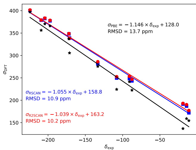
Fig. 2 ^{19}\text{F} magnetic shieldings, \sigma calculated with the PBE (black), rSCAN (blue) and r 2 SCAN (red) functionals vs. experimental chemical shifts, \delta . For each functional the line of best fit is given.
