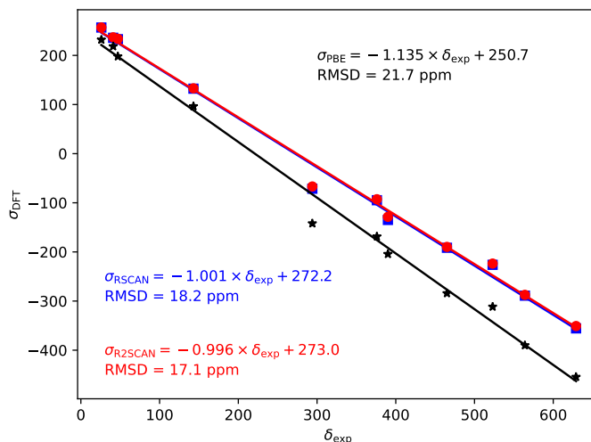
Fig. 3 ^{17}\text{O} magnetic shieldings, \sigma calculated with the PBE (black), rSCAN (blue) and r 2 SCAN (red) functionals vs. experimental chemical shifts, \delta . For each functional the line of best fit is given.
