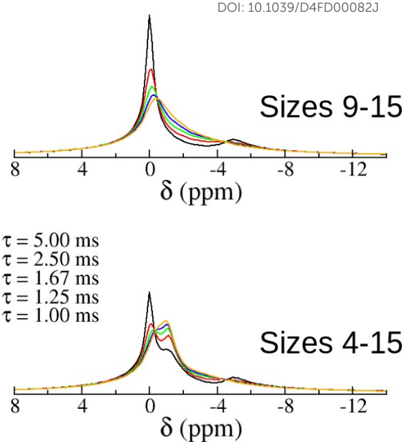
Fig. 6 NMR spectra calculated for the "different-size" configuration, for an in-pore chemical shift of -5 ppm for all particle sizes and correlation times.
