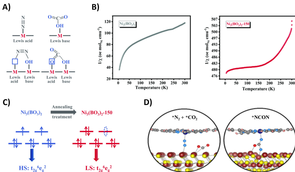
Fig. 21 Mechanistic investigations regarding CO_2 and N_2 activation using the Ni_3(BO_3)_2 -150 (A)–(C) and CoPc– MoS_2 catalyst (D). (A) Schematic illustration of adsorption of CO_2 and N_2 on frustrated Lewis pairs. (B) Temperature-dependent inverse susceptibility 1/\chi plots for pristine Ni_3(BO_3)_2 and Ni_3(BO_3)_2 -150 catalyst. (C) Schematic illustration of the spin-state regulation of Ni_3(BO_3)_2 after annealing treatment. (D) Schematic illustration of N_2 and CO_2 activation (left) and ^*NCON formation (right) on the CoPc– MoS_2 catalyst. Adapted from ref. 207 (A)–(C) and 205 (D), respectively.
