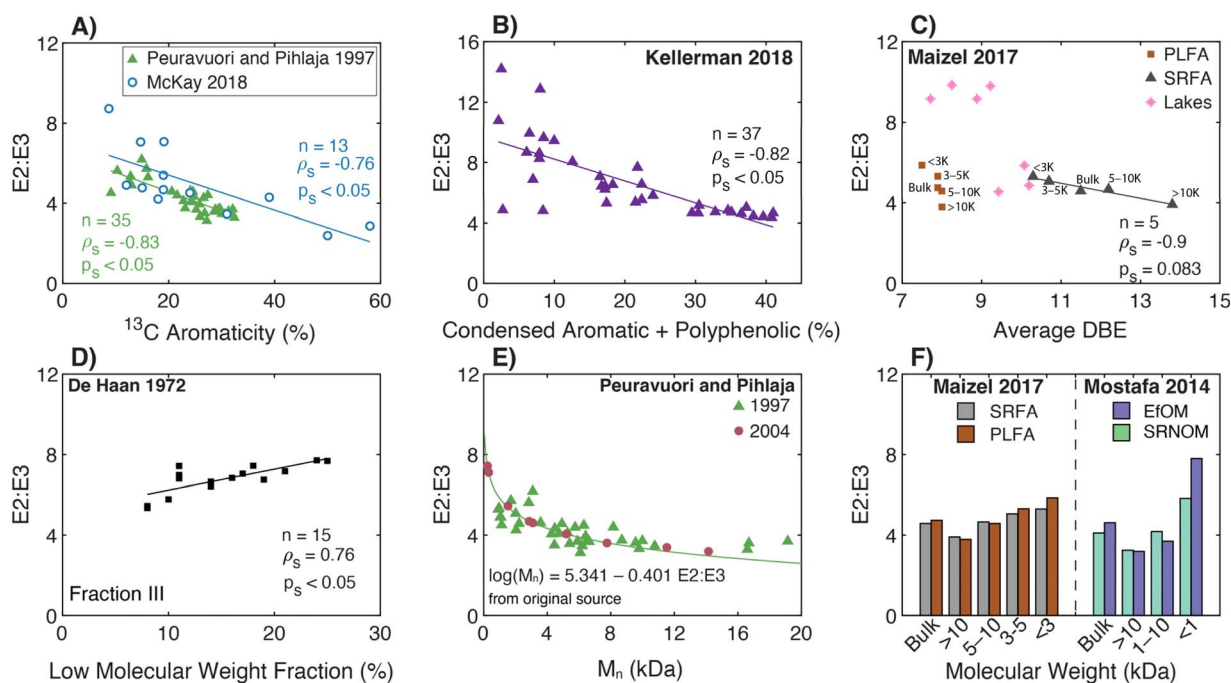
Fig. 5 Relationship between E2:E3 ( A_{250}/A_{365} ) and either molecular weight or different measures of aromatic carbon. (A) E2:E3 versus aromaticity (%) per sample calculated from 13 C NMR data. 39–43,155 (B) E2:E3 versus the relative abundance of condensed aromatic and polyphenolic formulae (%) per sample calculated based on Al_{mod} 132 from FT-ICR MS data. 35 (C) E2:E3 versus average double bond equivalents (DBE) calculated based on FT-ICR MS data for UF fractionated isolates (PLFA and SRFA) 36 and seven different lakes in northern Wisconsin of diverse trophic status. 37 (D) E2:E3 of the whole-water versus the percentage of low molecular weight DOM (longest retention time) for a lake. 156 (E) E2:E3 versus number-average molecular weight ( M_n ) for DOM from Nordic surface waters (humic substances and ultrafiltered samples). 155,188 (F) E2:E3 versus nominal molecular weight fractions for endmembers following UF fractionation. 36,38
