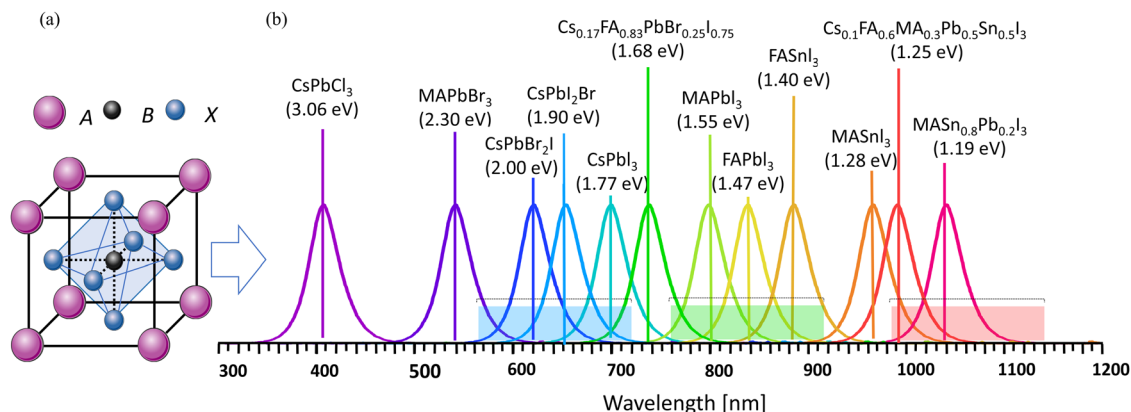
Fig. 7 (a) \text{ABX}_3 structure of perovskite material where A is a monovalent organic or inorganic cation such as methylammonium (MA), formamidinium (FA), and cesium (Cs). B is typically divalent lead (Pb) or tin (Sn) and X is a halide, mostly iodide (I) and bromide (Br) or a combination of them. (b) Perovskite bandgap tunability in the range from 1.2 eV to 3.1 eV. The bandgap range suitable for top cell, middle cell and bottom cell are highlighted by blue, green and red background accordingly. Adapted with permission from ref. 40 and 47 Copyright © 2020 Elsevier Inc and ref. 47 available from: https://doi.org/10.1021/nl5048779 , Copyright © 2019 American Chemical Society.
