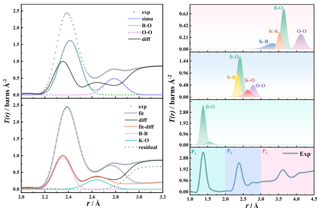
Fig. 2 Real spatial distribution function T(r) of 0.1\text{K}_2\text{O}\cdot 0.9\text{B}_2\text{O}_3 glass. Left panel: the fitting of peak P_2 , where the top figure shows the simulated B–O and O–O peaks, while the lower figure shows the B–B and K–O peaks obtained by subtraction. Right panel: the fitted peaks P_1 , P_2 and P_3 .
