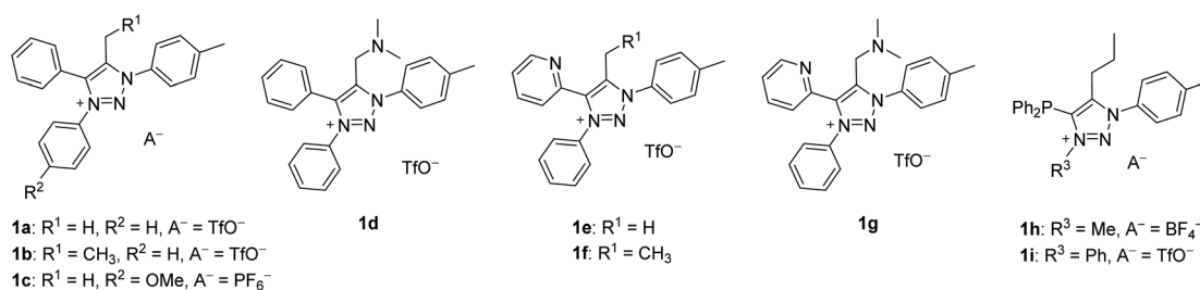
Fig. 3 The chemical structures of compounds 1a-i initially planned for the synthesis.
