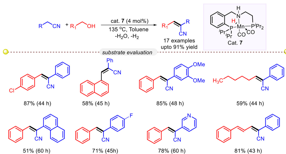
Scheme 12 An Mn-PNP catalyzed \alpha -olefination of nitriles with alcohols. 42
