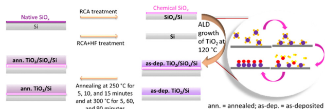
Fig. 1 Synthesis of TiO 2 on Si substrates by ALD using TiCl 4 and H 2 O as precursor materials.
