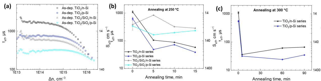
Fig. 2 (a) Injection-level dependent effective lifetimes for Si wafers passivated by 54 nm thin films of (a) as-deposited TiO 2 , (b) annealed TiO 2 films at 250 °C, and (c) annealed TiO 2 films at 300 °C for different durations. The corresponding surface recombination velocities ( S_{\text{eff}} ) are also shown on the right y-axis.
