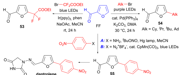
Scheme 17 Functionalisation of FF using radical-mediated photochemical processes.
