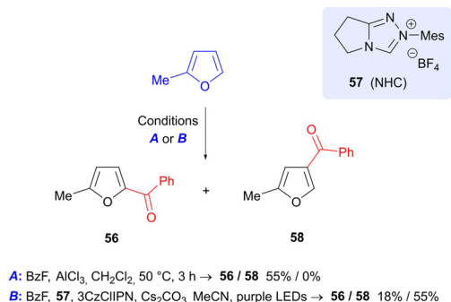
Scheme 18 Regioselective benzoylation of 2-methylfuran via Lewis-acid catalyzed and photochemical processes.
