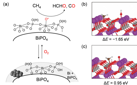
Fig. 14 (a) Proposed mechanism for \text{CH}_4 oxidation over \text{BiPO}_4 catalyst. DFT calculation for H abstraction from \text{CH}_4 by (b) the O atom adsorbed on surface Bi and (c) the lattice O atom. (Reproduced from ref. 52 with permission from Royal Society of Chemistry).
