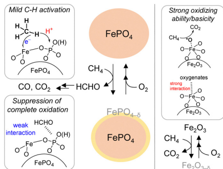
Fig. 13 Proposed reaction mechanism for oxidation of \text{CH}_4 over \text{FePO}_4 into \text{HCHO} with \text{O}_2 using \text{FePO}_4 and complete oxidation of \text{CH}_4 over \text{Fe}_2\text{O}_3 into \text{CO}_2 with \text{O}_2 using \text{Fe}_2\text{O}_3 . (Reproduced from ref. 53 with permission from Royal Society of Chemistry).
