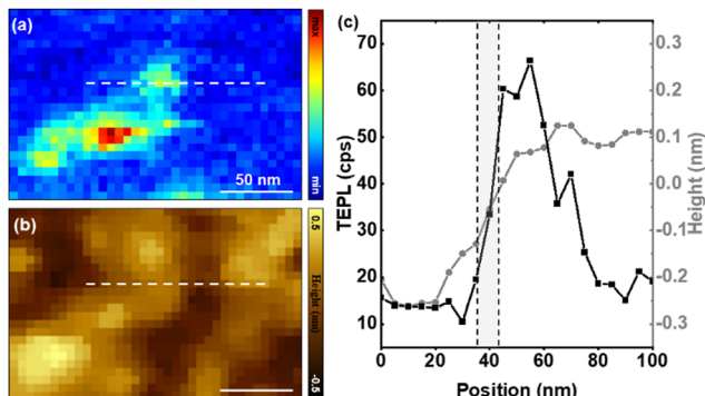
Fig. 4 Simultaneously recorded selected area TEPL (at 1.87–1.99 eV) and AFM maps (b) are shown. TEPL and AFM cross-sectional cuts taken along the dashed lines in (a) and (b) are shown on the same plot in (c). Conditions: 532 nm continuous wave laser source, 50 \mu W at the sample position, 0.5 s integration time at each pixel, 5 nm lateral/vertical steps in (a).
