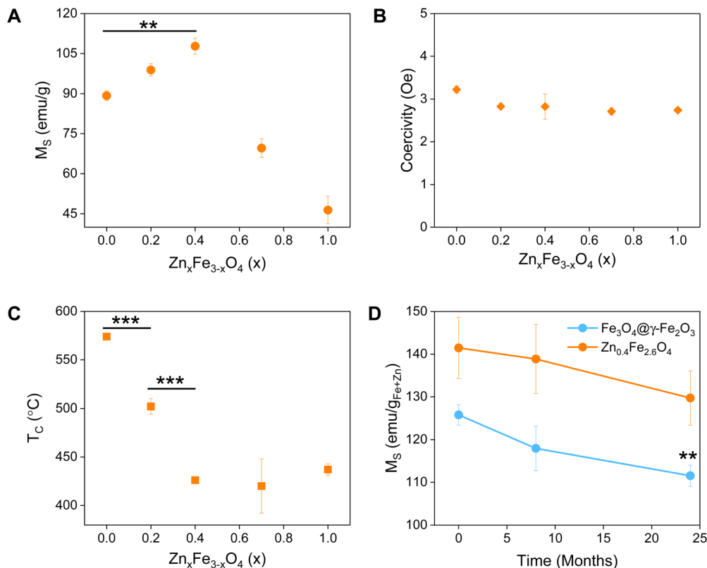
Fig. 3 Different properties of synthesized Fe_3O_4@γ-Fe_2O_3 and ferrites with various levels of Zn^{2+} doping: (A) saturation magnetization in emu g_{sample}^{-1} ( M_s ); (B) coercive field; (C) Curie temperature ( T_C ); and (D) long-term monitoring of the M_s , values were compared between 0 and 24 month for Fe_3O_4@γ-Fe_2O_3 . Values reported as mean \pm SEM, n = 3 , p values were calculated based on a two-tailed t test: *** indicates p < 0.001 , ** indicates p < 0.01 and * indicates p < 0.05 .
