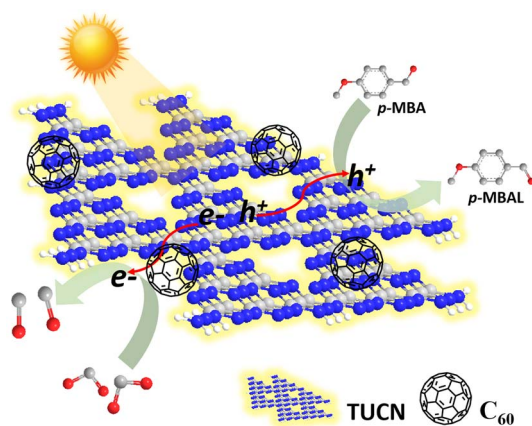
Scheme 2 Plausible mechanistic illustration of dual photoredox CO 2 reduction to CO coupled with p -MBA oxidation over the 5-C 60 /TUCN photocatalyst.
