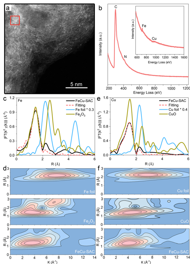
Fig. 2 (a) HAADF-STEM image of FeCu-SAC. (b) EELS spectrum for FeCu-SAC (inset: magnified spectrum and fitting for Fe and Cu peaks). (c) Fe K-edge EXAFS R space plot and fitting results for FeCu-SAC. (d) Fe K-edge EXAFS WT images of FeCu-SAC and references. (e) Cu K-edge EXAFS R space plot and fitting results of FeCu-SAC. (f) Cu K-edge EXAFS WT images of FeCu-SAC and references.
