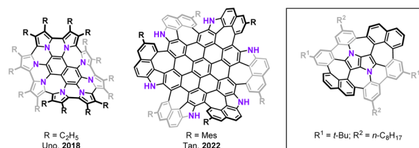
Fig. 1 Representative examples of negatively curved polyarenes containing multiple odd-membered rings.
