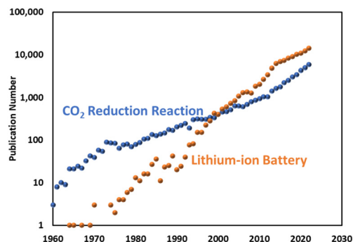
Fig. 1 Annual publications for an electrocatalytic CO 2 reduction reaction and lithium-ion battery research.
