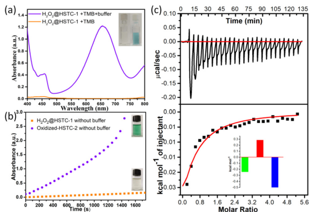
Fig. 5 (a) Comparison of the chromogenic reactions of \text{H}_2\text{O}_2 @HSTC-1 and HSTC-1 with TMB. The inset is a photograph of their TMB chromogenic reaction, respectively. (b) The time-dependent absorbance plots of \text{H}_2\text{O}_2 @HSTC-1 and oxidized-HSTC-2 after the addition of TMB solution without buffer. The inset is a photographic comparison of their TMB chromogenic reactions. (c) ITC thermogram of the titration of the HSTC-1 suspension (4 mM, 1.8 mL) with \text{H}_2\text{O}_2 (99 mM, 15 \mu\text{L} each injection) and fitting with a single-site model. The inset depicts the magnitude of the calculated thermodynamic parameters.
