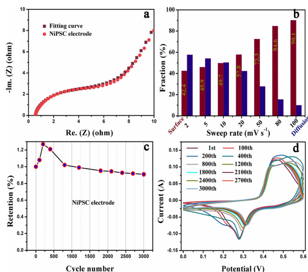
Fig. 3 Mechanism and cycling stability. (a) Nyquist plots of NiPSC. (b) Normalized contribution ratio of surface/diffusion-controlled currents at various scan rates. (c) Capacitance retention of NiPSC in the CV cycling test under the three-electrode system. (d) CV cycling test for NiPSC at 30 mV s -1 for 3000 cycles.
