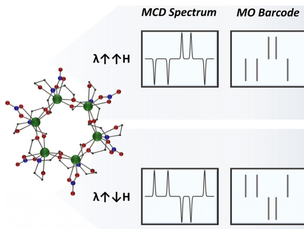
Scheme 1 (Left) Crystal structure of [\text{Er}_6(\text{teaH})_6(\text{NO}_3)_6] \cdot 6\{\text{Er}_6\} (colour code: green (Er); red (O), blue (N), black (C)) MCA (CCDC number: 1876163). (Right) representation of the dual-signalled magneto-optical barcode obtained via MCD spectroscopy.
