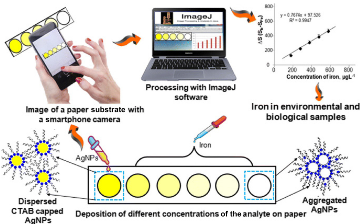
Fig. 3 Design and development of a smartphone-assisted paper-based portable colorimetric device for the on-site detection of the analyte [this figure has been reproduced from ref. 44 with permission from Springer Nature, copyright 2020].
