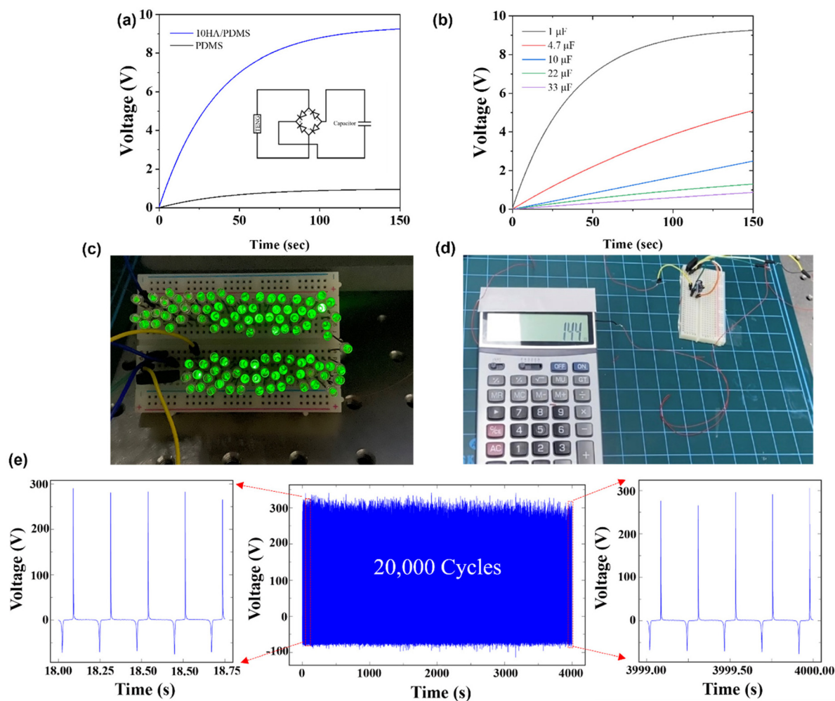
Fig. 5 (a) The charging curves of a 1\ \mu\text{F} capacitor comparing PDMS and optimal 10HA/PDMS at an input frequency of 5 Hz and an applied force of 2 N. (b) The charging curves of different capacitors with optimized 10HA/PDMS at an applied force of 2 N. (c and d) HA-TENG powering 100 LEDs or a commercial calculator. (e) Endurance test of the optimized HA-TENG for more than 20 000 cycles.
