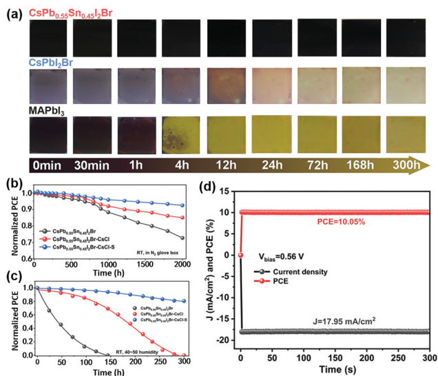
Fig. 4 (a) Photographs of \text{CsPb}_{0.55}\text{Sn}_{0.45}\text{I}_2\text{Br} , \text{CsPbI}_2\text{Br} and \text{MAPbI}_3 perovskite films under iso-thermal annealing ( 150^\circ\text{C} ) in an \text{N}_2 -filled glove box. The long-term normalized PCE of PSCs (b) in an \text{N}_2 -filled glovebox and (c) in the ambient air (40–50% RH). (d) MPPT of a \text{CsPb}_{0.55}\text{Sn}_{0.45}\text{I}_2\text{Br} -CsCl-S-based device. Reproduced from ref. 68 with permission from Wiley-VCH. Copyright 2021.
