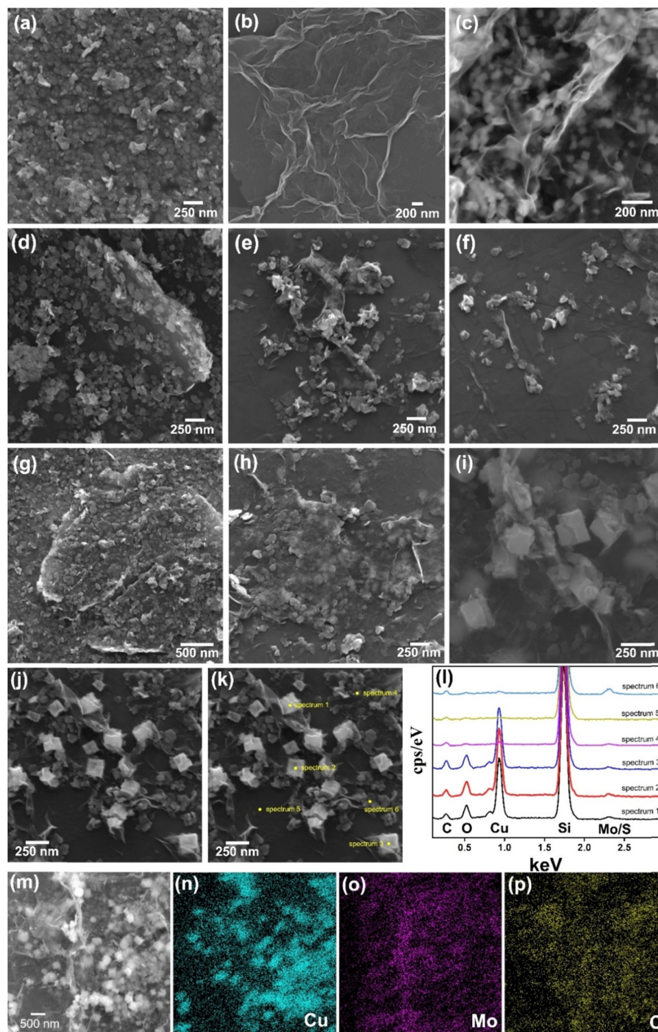
Fig. 3 Scanning electron microscopy images of MoS 2 (a); rGO (b); rGO/Cu x O (c); rGO/MoS 2 -LbL (d); rGO/MoS 2 -mixing (e); rGO/MoS 2 - in situ (f); rGO/Cu x O/MoS 2 -LbL (g); rGO/Cu x O/MoS 2 -mixing (h); and rGO/Cu x O/MoS 2 - in situ (i). Energy dispersive spectroscopy data (j–p) of rGO/Cu x O/MoS 2 - in situ , including point analysis (j–l) and mapping (m–p).
