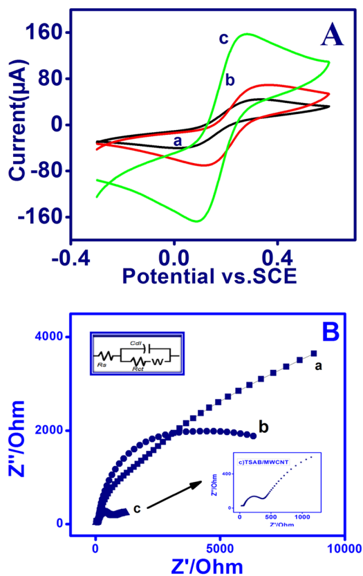
Fig. 2 (A) Cyclic voltammetry and (B) electrochemical impedance spectra on PIGE (curve a ), MWCNT (curve b ) and TSAB/MWCNT (curve c ) in 1 mM [\text{Fe}(\text{CN})_6]^{-3/4-} containing 0.1 mol \text{L}^{-1} ABS (pH-5.0) at 50 \text{mV s}^{-1} . Inset: Enlarged image of (B) depicting the EIS of TSAB/MWCNT-modified electrode.
