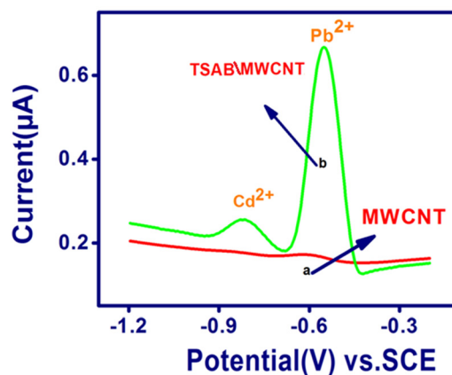
Fig. 3 SWASV performed on MWCNT (A) and TSAB/MWCNT (B) with \text{Pb}^{2+} and \text{Cd}^{2+} (8 ppb) accumulated on electrode surface in 0.1 M acetate buffer solution (pH 5.5).
