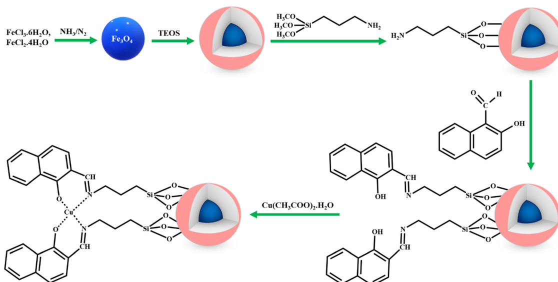
Scheme 18 Preparation of \text{Fe}_3\text{O}_4@(\text{SiO}_2)_x /Schiff base/Cu nanocatalyst.
