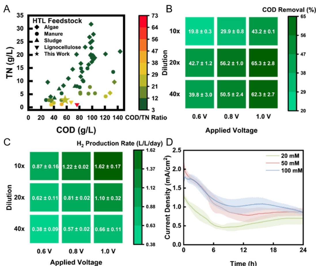
Fig. 1 (A) COD/TN composition of feedstock PHW used in this study and other PHW studies. Literature data were collected from Watson et al. (2020). 27 The COD removal (B) and \text{H}_2 production rate (C) of PHW-fed MEC in 3-day period under different applied voltage and dilution ratio. (D) The current density profile under different buffer strength after introduction of fresh electrolyte. The shadows represent standard deviation from triplicate experiments.
