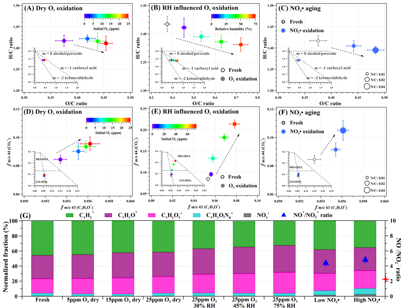
Fig. 1 HR-ToF-AMS measured chemical transformations of HULIS aerosols following dry ozonolysis (A and D), RH-dependent \text{O}_3 oxidation (B and E) and \text{NO}_3^\bullet -dominated heterogeneous aging (C and F). The plots show Van Krevelen (VK) diagrams, organic elemental ratios (A–C), and triangle plots of f_{43} vs. f_{44} (D–F). Panel G shows the ensemble-normalized fragments' compositions. A V–K plot is inserted in panel A–F. The dashed triangle zone in panel D–F constrains ambient oxygenated organic aerosol (OOA), two specific regions classify the oxidation level of OOA (less- and more-oxidized OOA, LO-OOA vs. MO-OOA). In panels A–F, the dashed arrows indicate the chemical trends with increasing \text{O}_3 , RH and \text{NO}_3^\bullet . \text{NO}^+/\text{NO}_2^+ ratios in \text{NO}_3^\bullet oxidized HULIS were specifically displayed as solid blue triangle in panel G. The red star at the right-hand Y-axis indicates \text{NO}^+/\text{NO}_2^+ ratio of 2.1 for \text{NH}_4\text{NO}_3 aerosols measured by the AMS.
