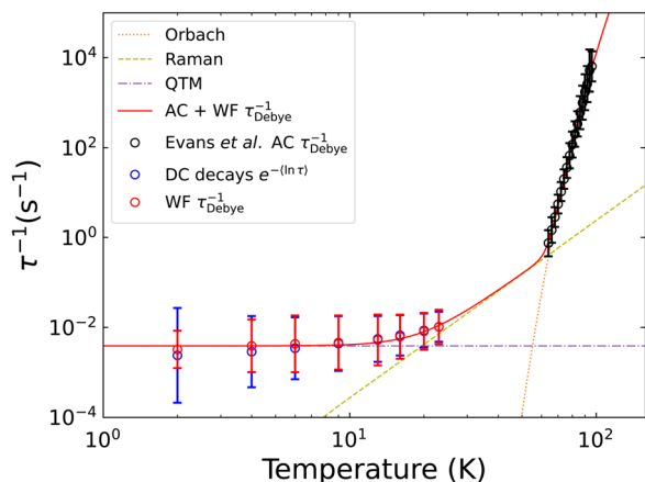
Fig. 5 Comparison of \tau_{\text{Debye}}^{-1} and e^{-(\ln|\tau|)} extracted from Waveform and DC decay measurements of [\text{Dy}(\text{Dtp})_2][\text{Al}\{\text{OC}(\text{CF}_3)_3\}_4] . The waveform (red) and AC data [22] (black) are fitted to eqn (10), with each contribution represented as a dotted line. Fitted parameters are given in Table 2.
