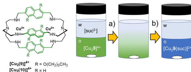
Fig. 9 Schematized structures of the dicopper cryptates of cages 9 and 10 , and application of [Cu 2 (9)] 4+ as extractant for succinate 76 from aqueous solutions (0.05 mol L -1 HEPES buffer, pH = 7) into dichloromethane. The transfer of succinate into the organic phase and its binding into the cryptate cavity are accompanied by a change of colour in the organic phase, from green to blue.
