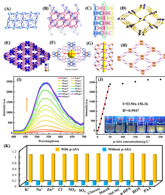
Fig. 5 (A)–(D) Crystal structure of Cu(I)-tpt; (A) coordination mode of Cu(I) with triazole unit of tpt ligand; (B) coordination mode of Cu(II) with triazole unit of tpt ligand; (C) 3D framework structure of Cu(I)-tpt and (D) sra network topology of Cu(I)-tpt. (E)–(H) Crystal structure of Cu(II)-tpt; (E) 3D framework structure of Cu(II)-tpt and (F) its rhombus channels of 17.6 Å × 12.4 Å; (G) 1D channels of Cu(II)-tpt; (H) ant network topology of Cu(II)-tpt; (I) the changes in fluorescence emission spectra of the Cu(II)-tpt-on-Cu(I)-tpt membrane after mixing concentration of p -ASA (0–200 \mu\text{g L}^{-1} ); (J) corresponding line relationship between emission intensity at \lambda_{540} and p -ASA concentrations (inset: corresponding photographs under UV lamp); (K) competitive binding ability of the Cu(II)-tpt-on-Cu(I)-tpt membrane toward various analytes. Reprinted with permission from ref. 69. Copyright 2020 American Chemical Society.
