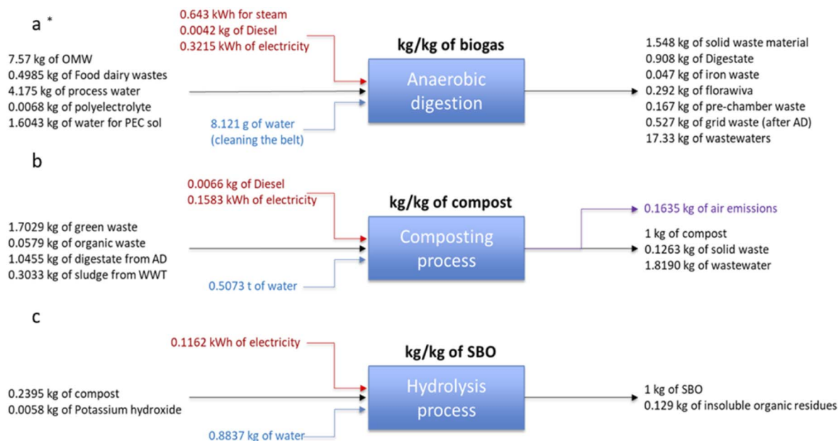
Fig. 12 Mass and energy input/output for the anaerobic digestion process in \text{kg kg}^{-1} of biogas (a), composting process in \text{kg kg}^{-1} of compost (b) and hydrolysis process in \text{kg kg}^{-1} of SBO (c). Legends: organic fraction of municipal solid waste (OMW); anaerobic digestion (AN); sludge waste water treatment section (WWT); soluble biobased product (SBO); insoluble organic residue accounted as unreacted compost.
