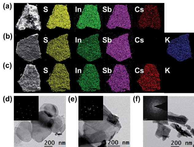
Fig. 2 Elemental mapping images of (a) Cs@NIAS, (b) KIAS, and (c) KIAS-Cs. TEM images of (d) Cs@NIAS, (e) KIAS and (f) KIAS-Cs; inset: the corresponding SAED patterns for d–f.
