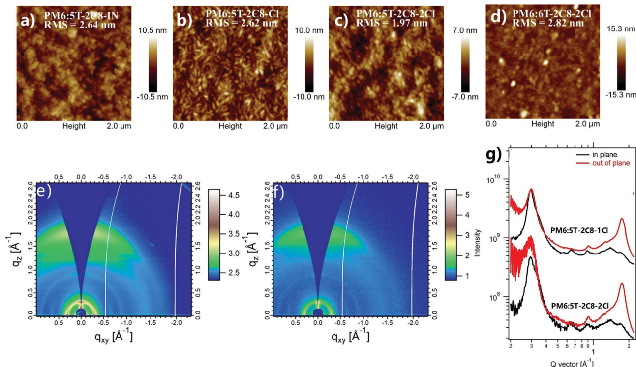
Fig. 3 AFM images of the blend films based on 5T-2C8-IN (a), 5T-2C8-1Cl (b) 5T-2C8-2Cl (c) and 6T-2C8-2Cl (d), the 2D GIWAXS patterns based on PM6:5T-2C8-1Cl (e) and PM6:5T-2C8-2Cl (f) and the corresponding line-cut profiles (g).
