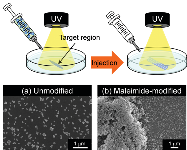
Fig. 7 SEM images of photo-assemblies of maleimide-P( St-co-MAA-co-MPC ) particles on (a) unmodified and (b) maleimide-modified glass substrates after the particles were injected into the substrate surface under UV irradiation.
