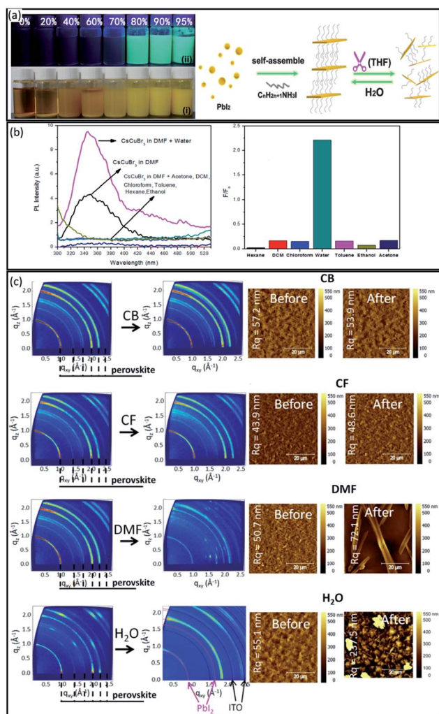
Fig. 9 (a) Photographs of solution/suspensions of (C_{16}H_{33}NH_3)_2PbI_4 with different water contents under ambient (i) light and (ii) UV-365 nm radiation, and schematic illustration of the solvent sensing mechanism of (C_{16}H_{33}NH_3)_2PbI_4 perovskite. Reproduced with permission from ref. 118, Copyright 2014 John Wiley and Sons. (b) Photoluminescence spectrum and solvent selectivity of the perovskite compound in the presence of various solvents. Reproduced with permission from ref. 131 Copyright 2016 Elsevier. (c) 2D GIXRD patterns and AFM images of MAPbI_{3-x}Cl_x films before and after different solvent exposure. Reproduced with permission from ref. 132 Copyright 2019 Springer.
