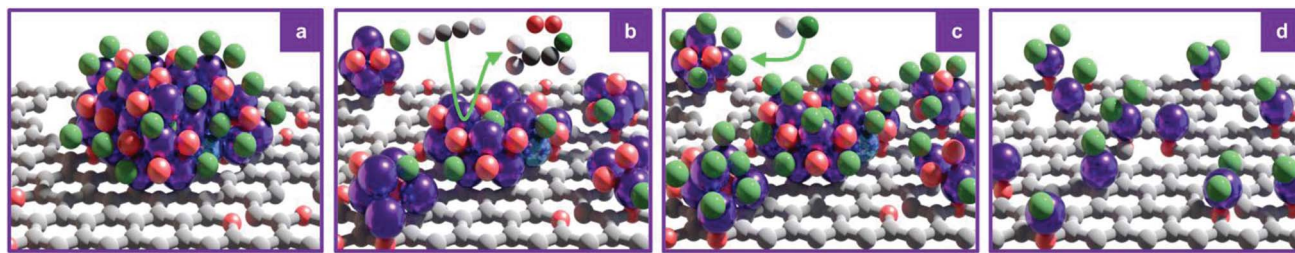
Fig. 5 Schematic representation of the \text{C}_2\text{H}_2 -induced redispersion mechanism of (a) \text{RuO}_x\text{Cl}_y NPs supported on carbon. (b) \text{C}_2\text{H}_2 reduces the NP surface, evolving VCM, depleting accessible surface Cl atoms, and \text{O}_2 while promoting Ru redispersion into smaller clusters or atoms. (c) Exposure to HCl leads to oxidative Cl addition, rechlorinating the cluster surface. (d) The alternating treatment is effective until full atomic dispersion is achieved. Colour code: purple = Ru, red = O, green = Cl, grey = C and white = H.
