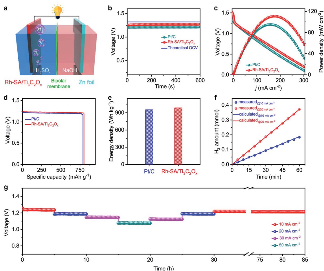
Fig. 5 Zn-H 2 battery hydrogen production system: (a) schematic illustration of the Rh-SA/Ti 3 C 2 O x -based Zn-H 2 battery hydrogen production system; (b) the open-circuit voltage curves; (c) the plots of polarization curves and the corresponding power densities; (d) the plots of voltage versus specific capacity at a scan rate of 10 mA cm -2 , where the specific capacity was normalized to the mass of consumed Zn; (e) plots of energy densities; (f) the amount of generated H 2 as a function of the reaction time at current densities of 10 and 20 mA cm -2 , respectively; (g) discharge curves of the hydrogen production system based on Rh-SA/Ti 3 C 2 O x with current densities from 10 to 50 mA cm -2 and the long-term stability tests at current densities of 10 mA cm -2 over 55 h.
